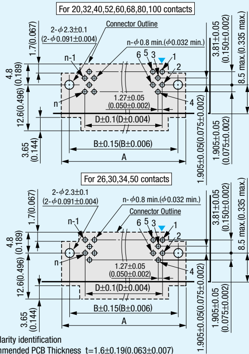
Printed Circuit Board Layout (Component Side View)
