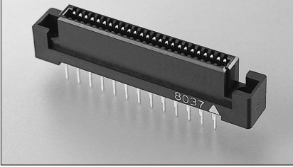
Receptacle (Straight Type)
